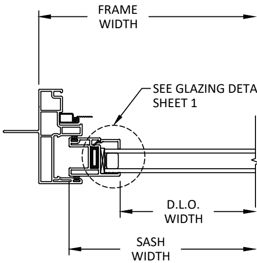
A HORIZONTAL SECTION 5 OPERABLE JAMB
