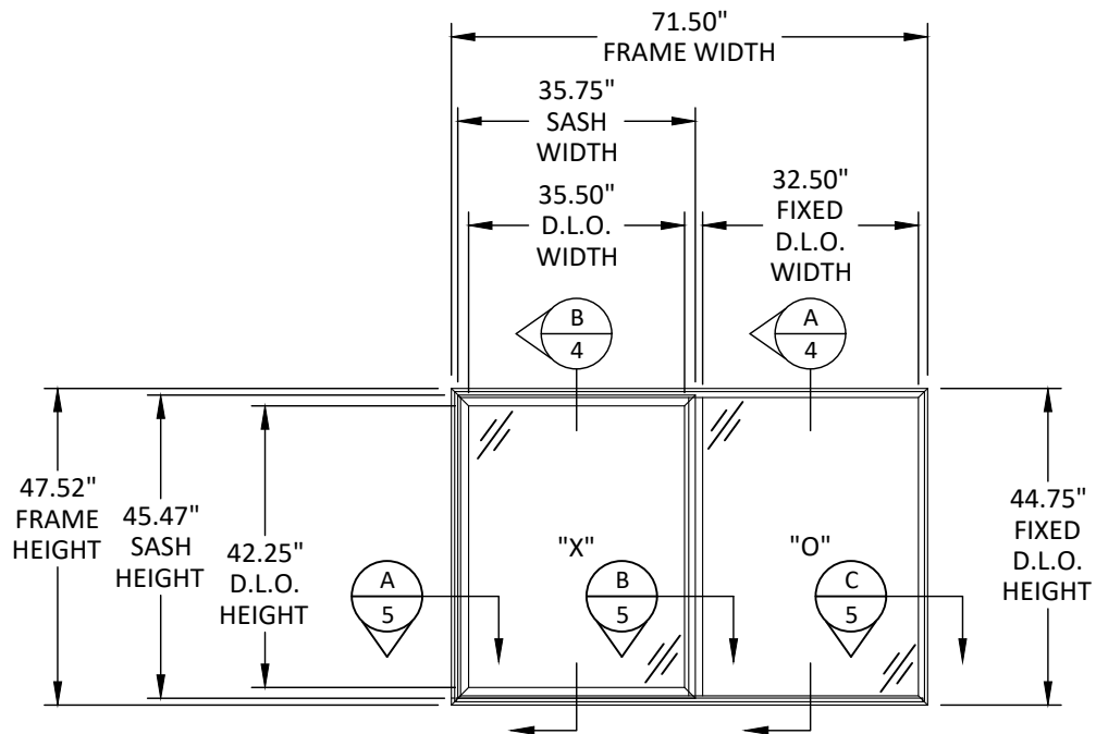
ELEVATION XO HORIZONTAL SLIDING WINDOW
