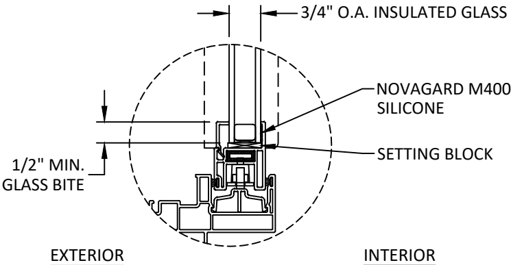
GLAZING DETAIL 1
