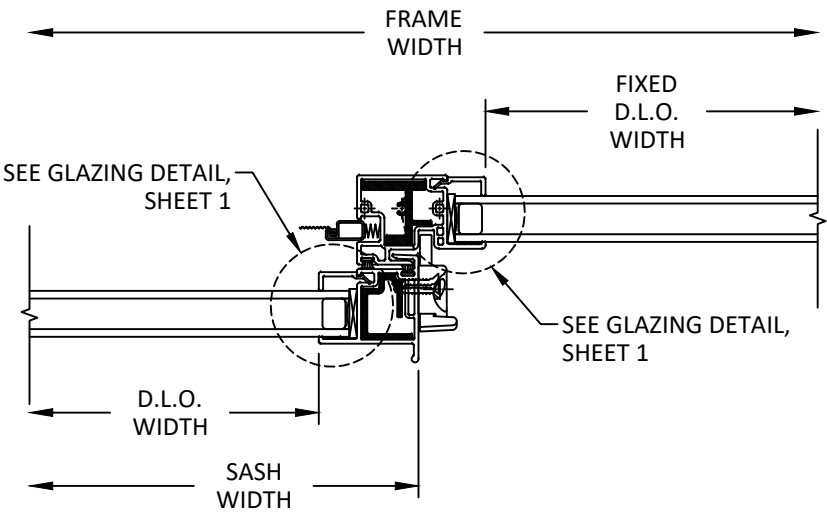
B HORIZONTAL SECTION 5 INTERLOCK
